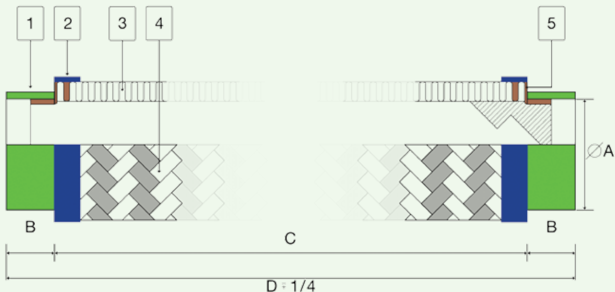
1:Tube End 2:Ferrule 3:Flexible 4:Wire 5:Brazed Joint
